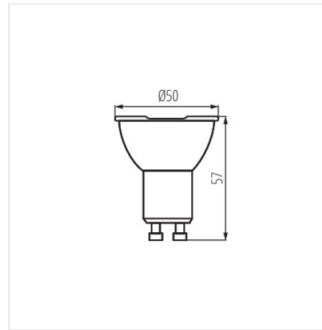
IQ-LED GU10 4,5W-NW
