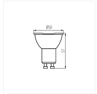
IQ-LED GU10 4,5W-CW
