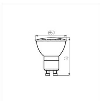
GU10 4W-NW LED
