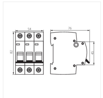
KMB6-C6/3
