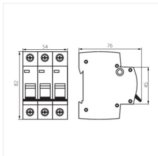
KMB6-C50/3
