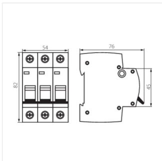
KMB6-C10/3
