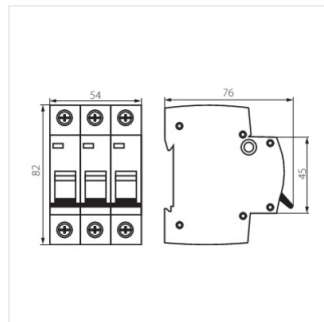
KMB6-C63/3
