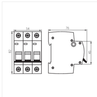
KMB6-C40/3
