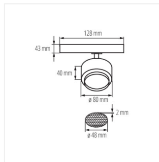
BTL 18W-930-B
