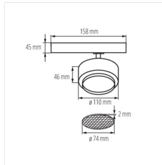
BTL 28W-930-B
